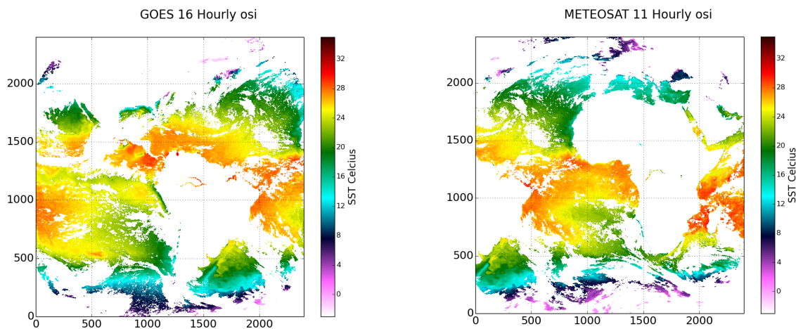
Figure 2: Geostationary chain SST products at 00:00 on the 30/1/2018; GOES-16 Figure 3: Geostationary chain SST products at 00:00 on the 30/1/2018; Meteosat-11
