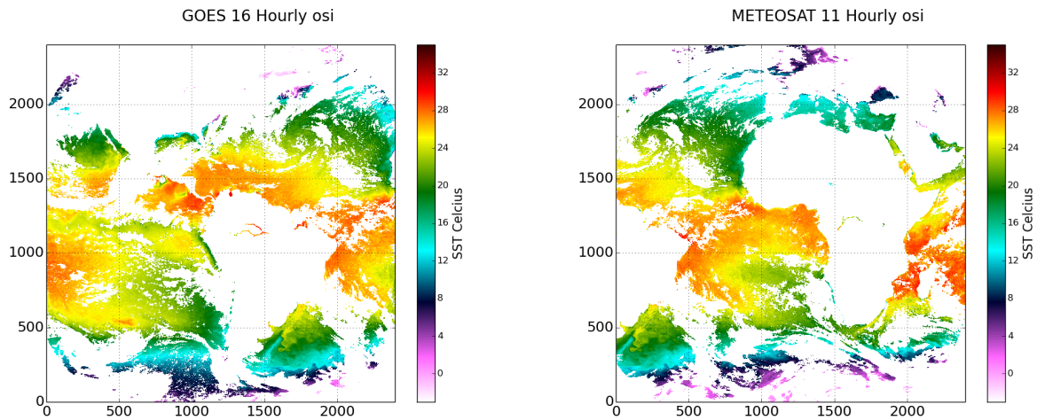
Figure 4: Geostationary chain SST products at 00:00 on the 30th of January 2018; left panels: GOES-16, right panels: Meteosat-11. Top panels: SST field derived from one frame at full resolution in satellite projection; middle panels: hourly collated files; bottom panels: hourly gridded fields.
